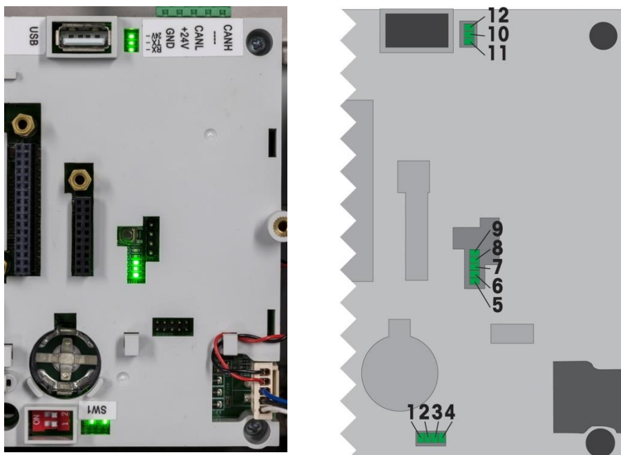
Figura 5-6: LEDs de placa principal POWERCELL
