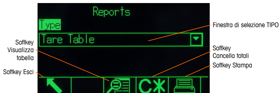
Figura 2-28: Schermata Report
